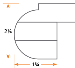
Triple Egg
