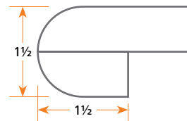
Double Bullnose
